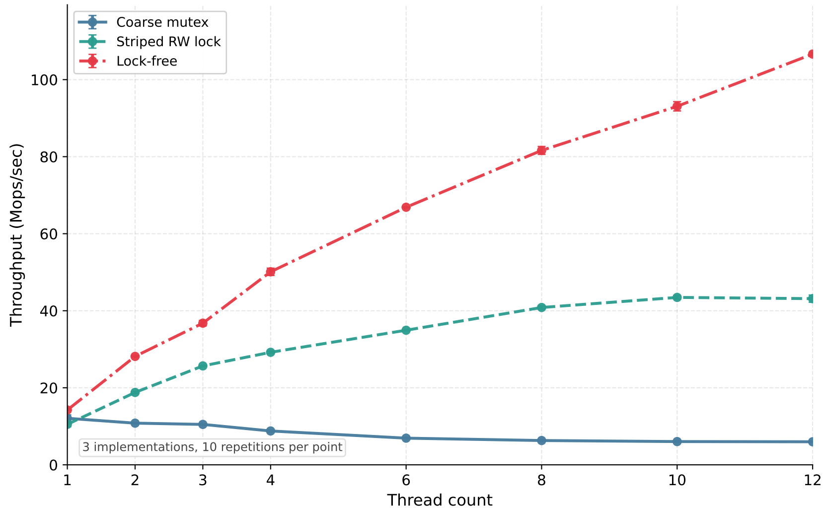
Concurrent Hash Table - Balanced mixed access
